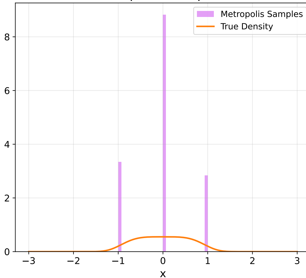
Random Walk (Step=1), Acceptance Rate=0.42
